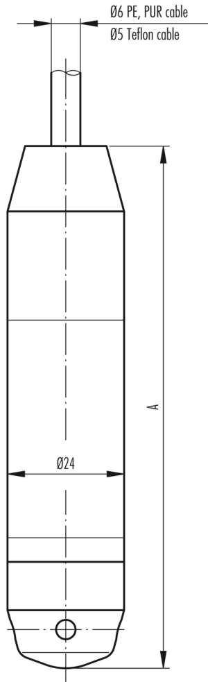
Fig. 1: Closed version
